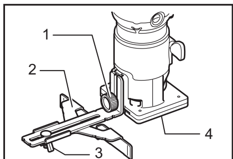
► 1. Clamp screw (A) 2. Straight guide 3. Wing nut 4. Base
